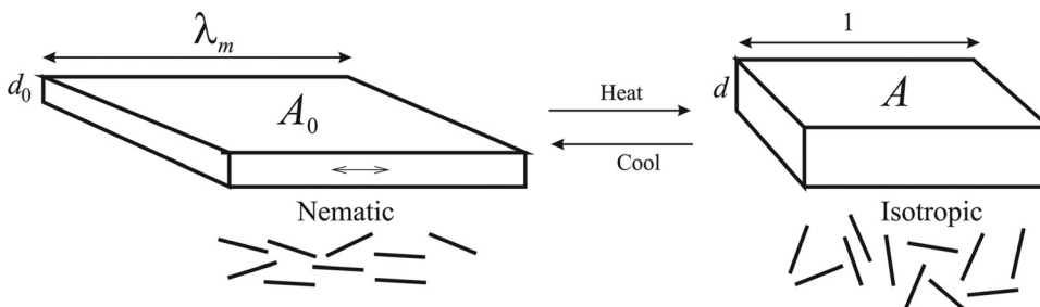
FIG. 6. Decrease of capacitance upon heating, with d = d_0\lambda and A = A_0/\lambda . C \propto A/d so \xi \propto \lambda^2 for a constant volume deformation.
