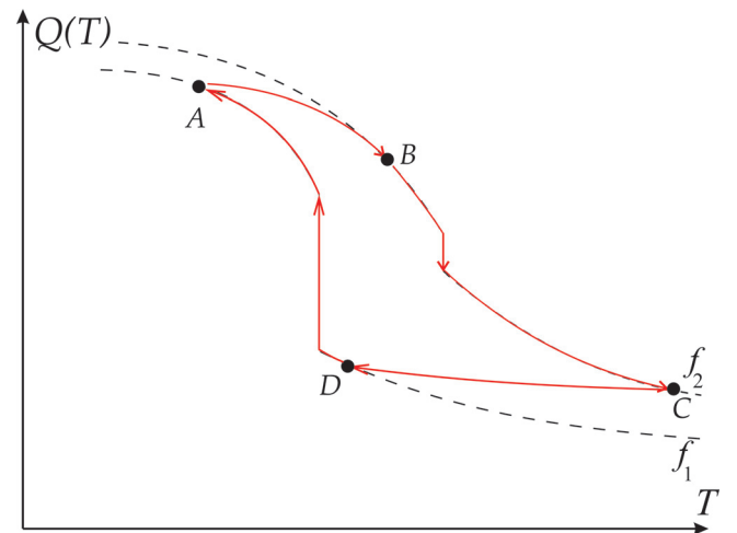
FIG. 5. (Color online) Schematic of a charge pump undergoing the cycle, described in Fig. 2, with reduced external fields f_1 and f_2 . Note resemblance to a conventional p-V diagram.
