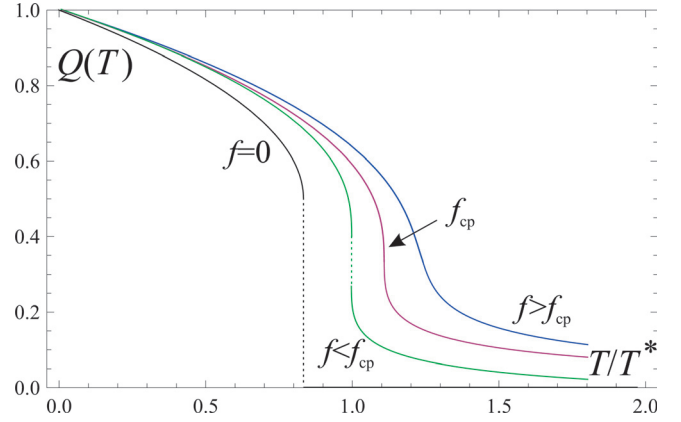
FIG. 4. (Color online) Order parameter vs temperature T generated by minimizing F_{nem}(Q) - fQ , where the linear term is the first order effect of an external field. Field strengths f are indicated. Note the discontinuous change in Q at T_{ni} disappears at the critical point, f_{cp} = b^3/27c^2 (Ref. 5).
