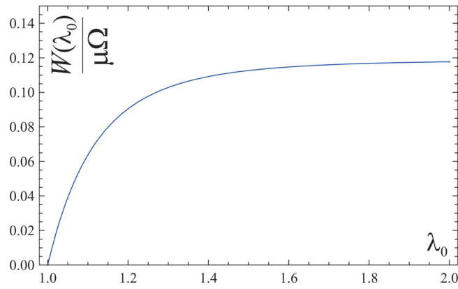
FIG. 11. (Color online) Optimal output, W_m/\mu\Omega , as a function of prestrain, \lambda_0 , and valid for \lambda_0 > 1.38 when v_w^{(1)} is used.
