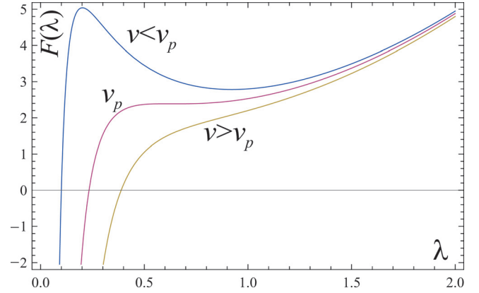
FIG. 8. (Color online) The free energy F_1(\lambda) for various reduced working voltages, v . For v < v_p , there is a clear minimum in free energy, disappearing for v > v_p , the lower plot. The limiting case, when the two extrema coincide, has F_1^{(1)}(\lambda_p) = F_1^{(2)}(\lambda_p) = 0 , which yields for rubber v_p = 3/4^{4/3} (Ref. 16).
