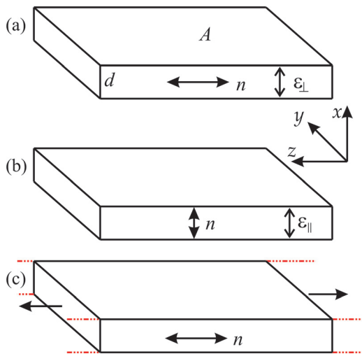
FIG. 7. (Color online) In each case, a capacitor with a LCE as the working substance - flexible electrodes are attached directly to the sample surfaces. The three proposed geometries: (a) director in plane, (b) director along x direction and (c) director in plane, with prestretch. The separation is d = d_0 \lambda where d_0 is the unstrained dimension. The volume, \Omega = Ad is conserved.
