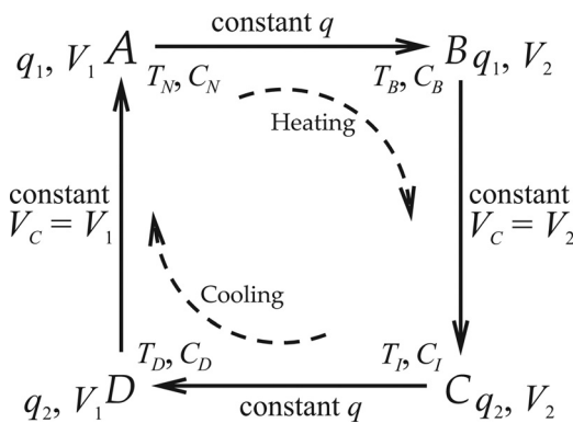
FIG. 2. Operating cycle of proposed charge pump. As temperature rises, capacitance drops, C_B < C_N , and since charge is constant, voltage rises to V_2 . Further increase in temperature decreases capacitance further, C_I < C_B , but charge can now flow out at the higher voltage V_2 . Cooling T_I \rightarrow T_D causes the capacitance to rise again, C_D > C_I , and the voltage drops to the point where charge can be received from the source at V_1 .
