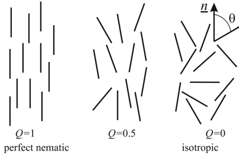
FIG. 3. Distribution of molecular axes around the average alignment direction, \underline{n} . Degree of ordering is quantified by the order parameter Q .
