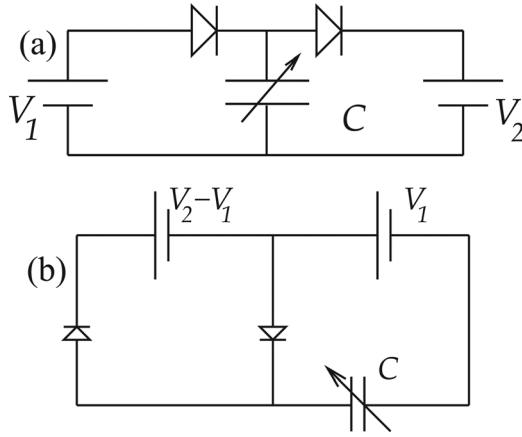
FIG. 1. (a) Charge pump: model circuit. Charge is pumped from the source V_1 to the higher voltage V_2 . (b) A more practical circuit which recharges the source battery.
