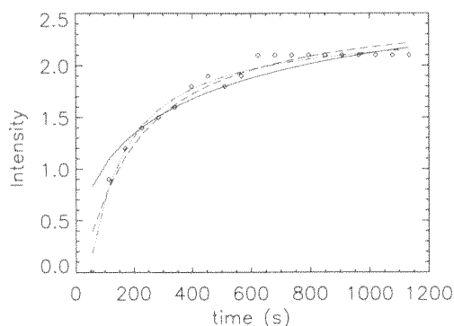
Fig. 6. Fit of preliminary data, indicated by diamonds, from Niu et al. [9] for T = 550 K. Also plotted are fits to the expressions in Eq. (1): solid curve; to Eq. (5): dashed curve; and to Eq. (4): dash-dotted curve.
