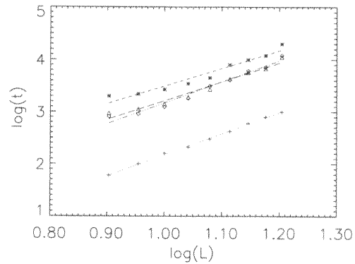
Fig. 4. Logarithm of the various time constants t vs. logarithm of the average distance L between single height steps (i.e., 1/\tan(\phi) ), where \phi is the misorientation angle), at T = 0.624\epsilon/k_B . The plus signs indicate the values of t_0 obtained by fitting Eq. (1) to our simulation results. The corresponding linear fit has a slope s = 4.36 \pm 0.06 . The asterisks, triangles, and diamonds indicate the values of t_1 , t_2 , t_3 , respectively, obtained by fitting Eq. (4) to our simulation data. The corresponding best linear fits are shown. Their respective slopes are 3.37 \pm 0.30 , 3.62 \pm 0.25 and 4.03 \pm 0.25 . This result and those of Bartelt et al. [17] suggest a relation of the form of Eq. (6).
