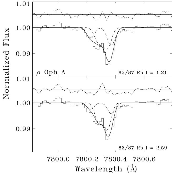
FIG. 1.—Rb I toward \rho Oph A. The best fit appears in the top panel, and a fit forcing the Rb isotope ratio to be the solar system value is in the bottom panel. Notice the lack of agreement in the shoulders of the line in the bottom panel. The dashed lines show the contributions from ^{85}\text{Rb} and the dot-dashed ones from ^{87}\text{Rb} . The line above each spectrum indicates data minus fit, offset to 1.005.
