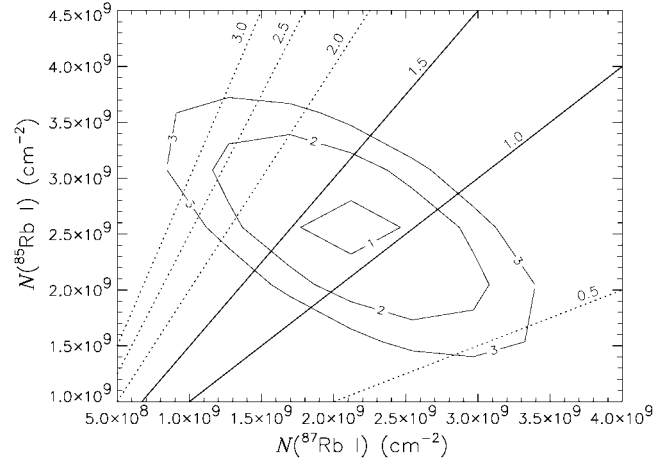
FIG. 2.—Map of \chi^2 confidence levels for the best fit to Rb I absorption. Contours for 1, 2, and 3 \sigma are shown. The straight lines shown as overlays represent different ^{85}\text{Rb}/^{87}\text{Rb} ratios.
