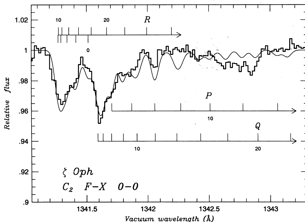
FIG. 3.—Spectrum of ζ Oph showing interstellar lines from the C 2 molecule's 0-0 band of the F-X system. Locations of the P , Q , and R branches are identified by the rotational quantum number J'' of the lower level. A synthetic spectrum computed as described in the text is represented by the solid line.
