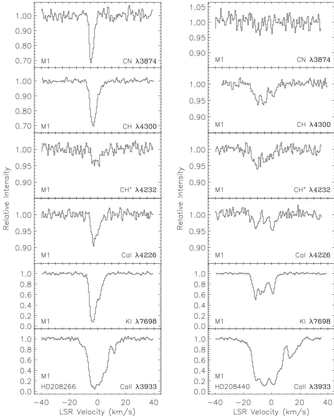
FIG. 9.—Interstellar CN, CH, CH + , Ca I, K I, and Ca II absorption profiles toward HD 208266 and HD 208440 (as for Fig. 1)
