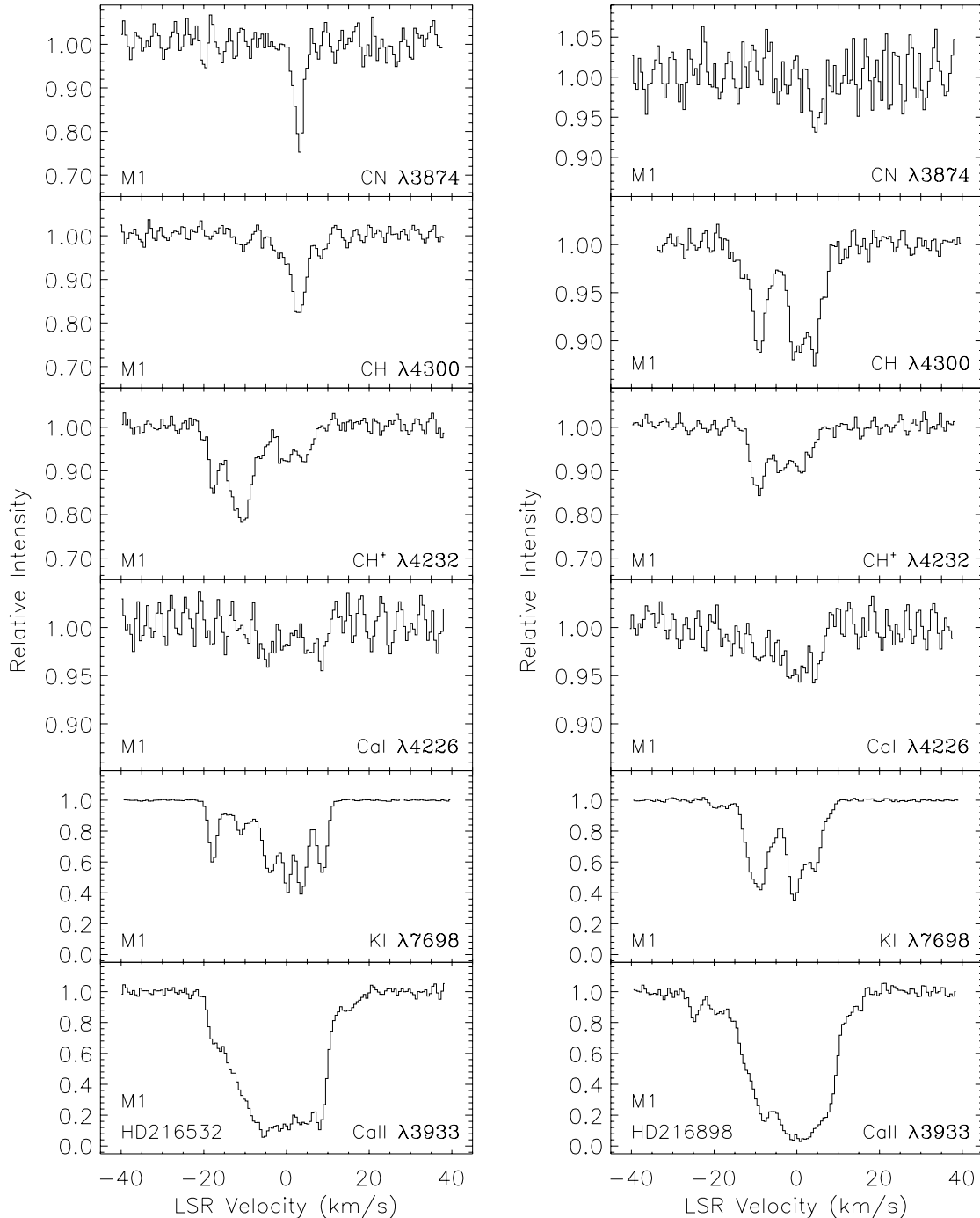
FIG. 13.—Interstellar CN, CH, CH + , Ca I, K I, and Ca II absorption profiles toward HD 216532 and HD 216898 (as for Fig. 1)
