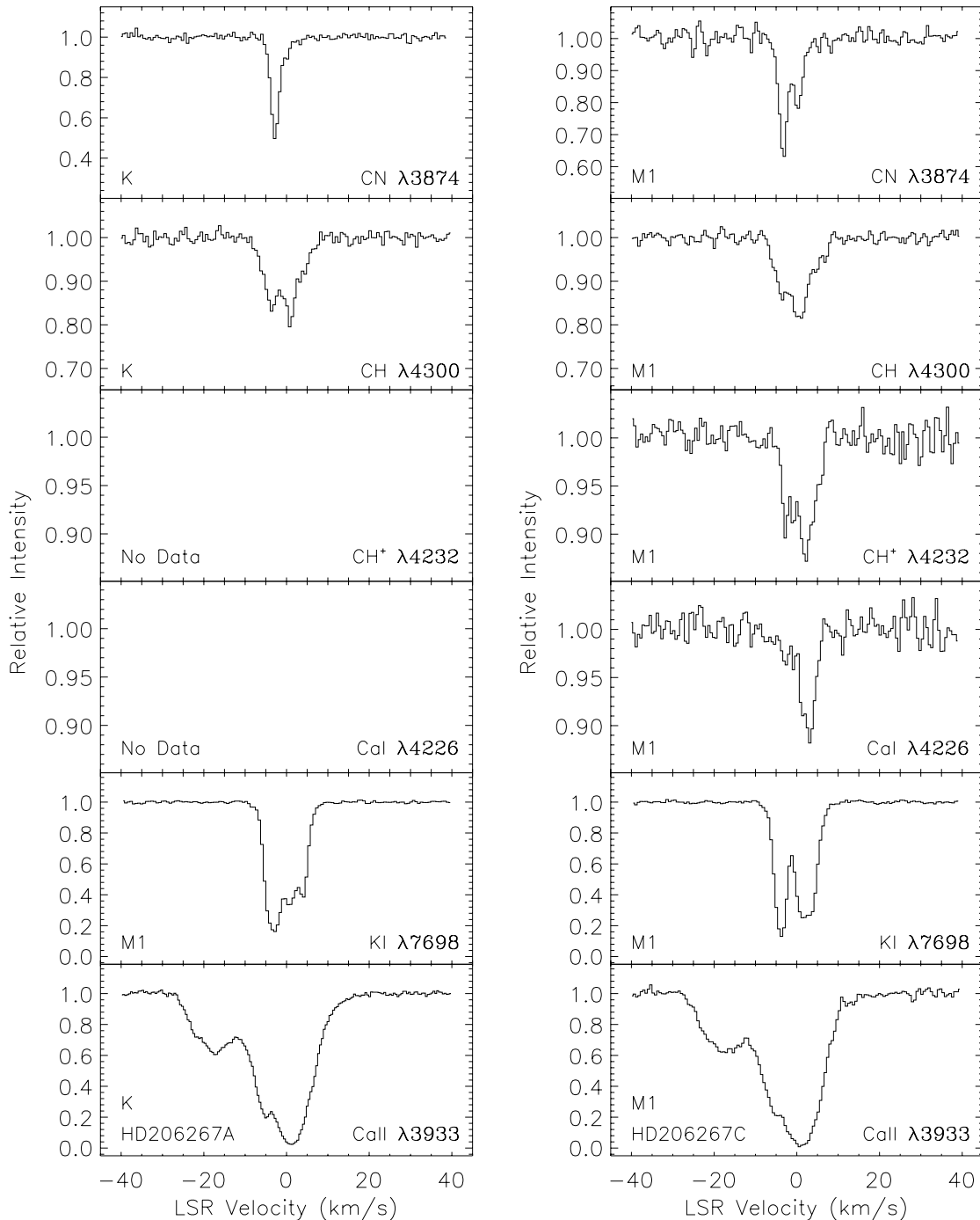
FIG. 5.—Interstellar CN, CH, CH + , Ca I, K I, and Ca II absorption profiles toward HD 206267A and HD 206267C (as for Fig. 1)
