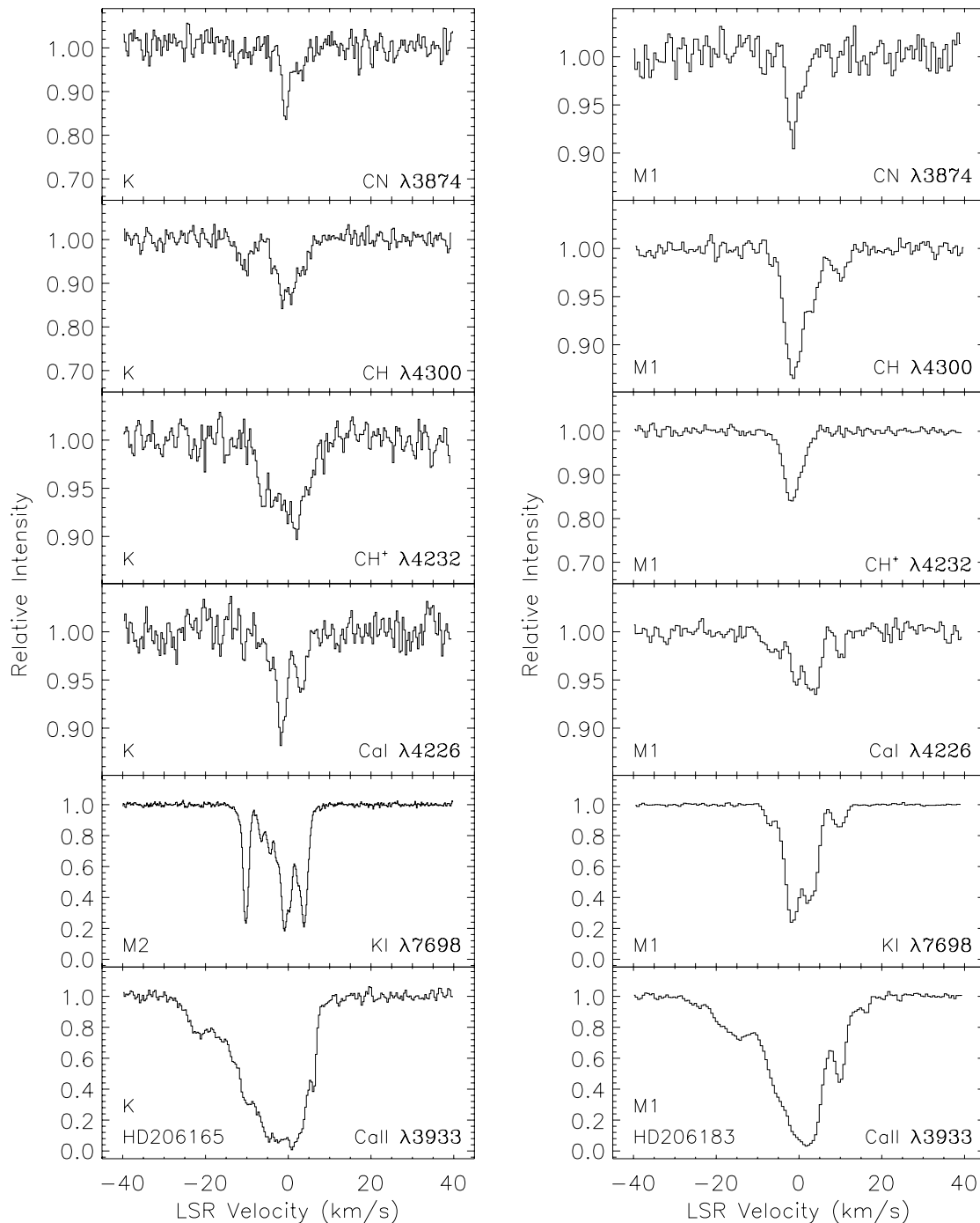
FIG. 4.—Interstellar CN, CH, CH + , Ca I, K I, and Ca II absorption profiles toward HD 206165 and HD 206183 (as for Fig. 1)
