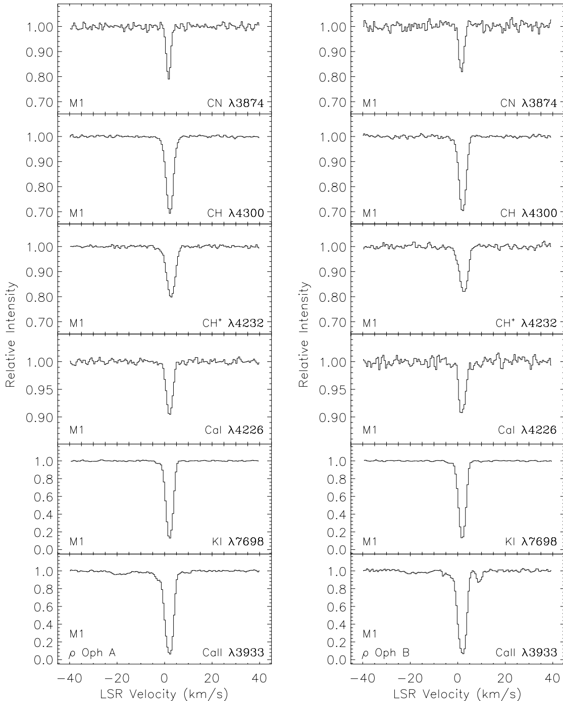
FIG. 1.—Interstellar CN, CH, CH + , Ca I, K I, and Ca II absorption profiles toward \rho Oph A and \rho Oph B. The transition is given in the lower right corner of each panel. The source of the spectra is denoted M1, M2, and K. M1 represents observations from McDonald Observatory during 2000 and 2001, whereas M2 denotes observations in 1995 and 1996 from McDonald Observatory with a higher resolution. All KPNO spectra are denoted K. Note that the vertical scales differ from panel to panel.
