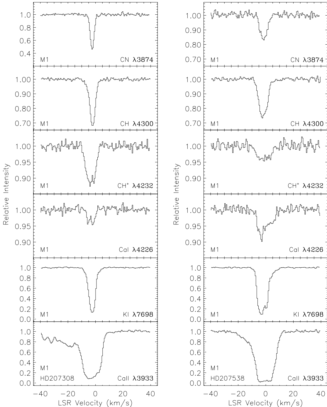
Fig. 8.—Interstellar CN, CH, CH + , Ca I, K I, and Ca II absorption profiles toward HD 207308 and HD 207538 (as for Fig. 1)
