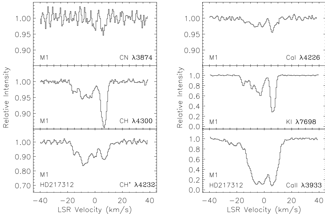
FIG. 15.—Interstellar CN, CH, CH + , Ca I, K I, and Ca II absorption profiles toward HD 217312 (as for Fig. 1)
