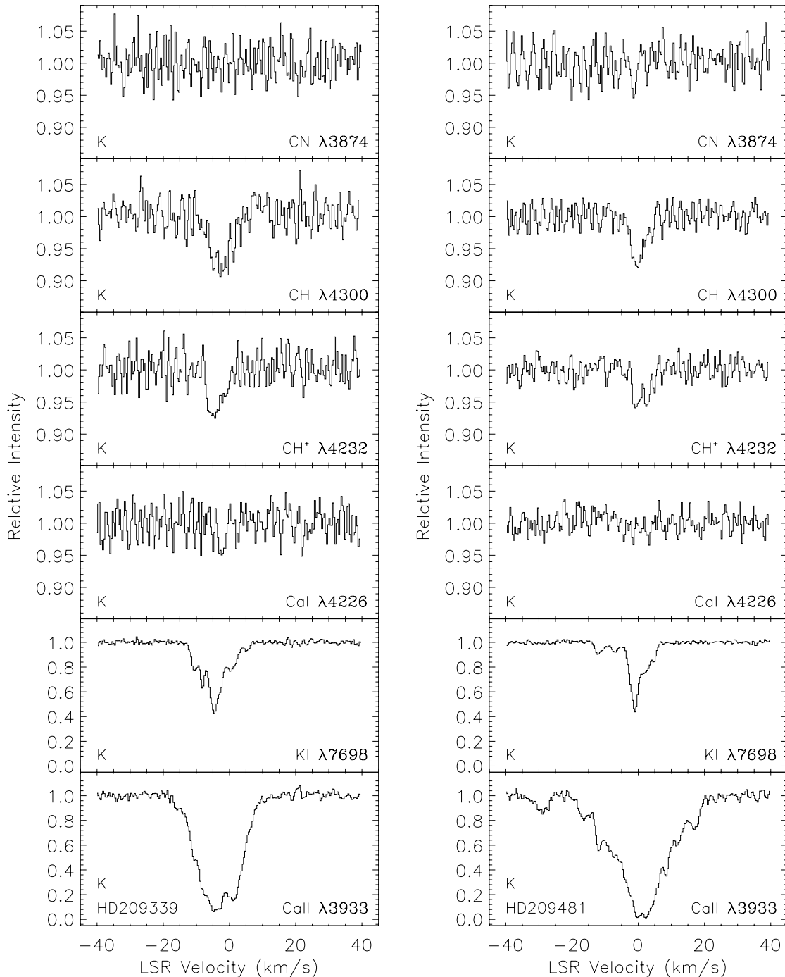
FIG. 11.—Interstellar CN, CH, CH + , Ca I, K I, and Ca II absorption profiles toward HD 209339 and HD 209481 (as for Fig. 1)
