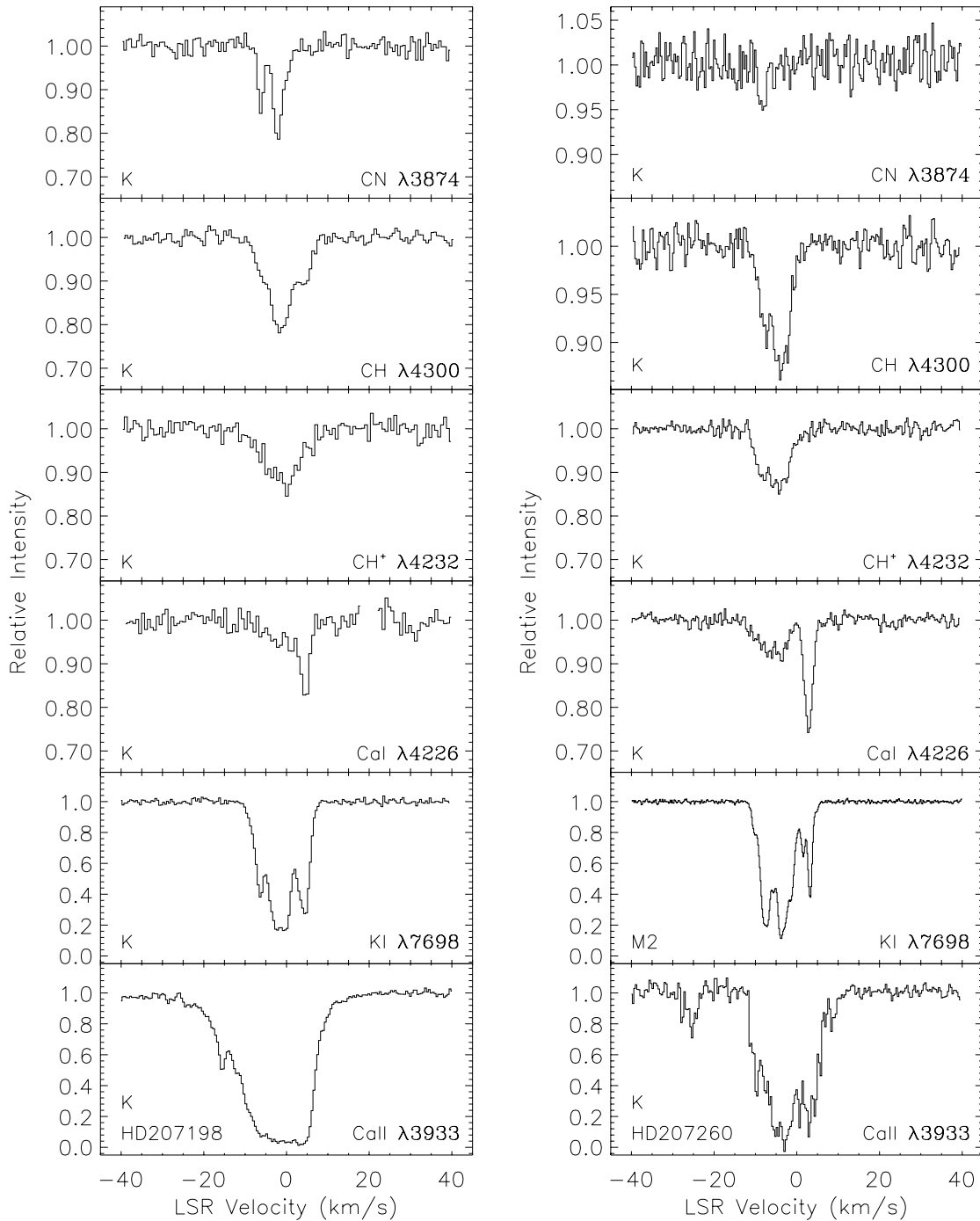
FIG. 7.—Interstellar CN, CH, CH + , Ca I, K I, and Ca II absorption profiles toward HD 207198 and HD 207260 (as for Fig. 1). Blank region for Ca I toward HD 207198 contains bad pixels.
