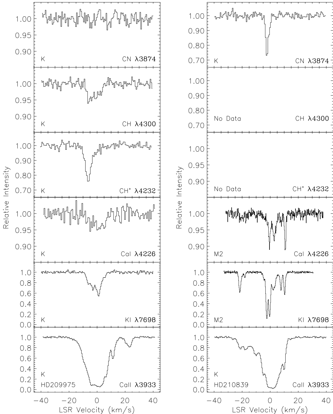
FIG. 12.—Interstellar CN, CH, CH + , Ca I, K I, and Ca II absorption profiles toward HD 209975 and HD 210839 (as for Fig. 1)
