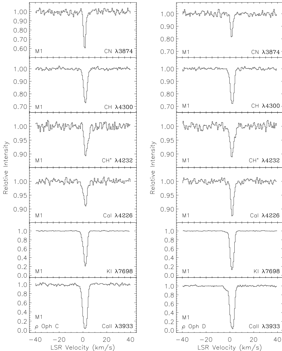
FIG. 2.—Interstellar CN, CH, CH + , Ca I, K I, and Ca II absorption profiles toward \rho Oph C and \rho Oph D (as for Fig. 1)
