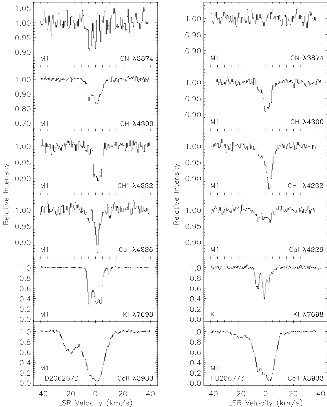
FIG. 6.—Interstellar CN, CH, CH + , Ca I, K I, and Ca II absorption profiles toward HD 206267D and HD 206773 (as for Fig. 1)
