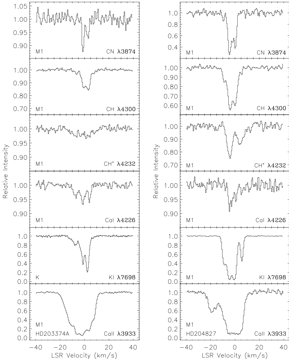
Fig. 3.—Interstellar CN, CH, CH + , Ca I, K I, and Ca II absorption profiles toward HD 203374A and HD 204827 (as for Fig. 1)
