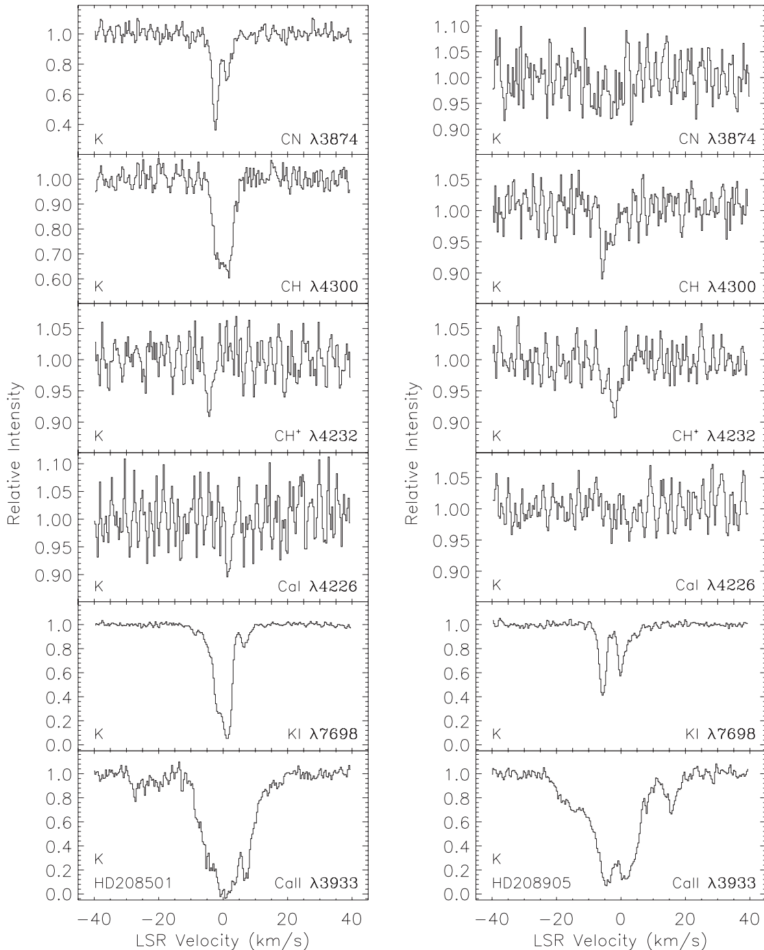
FIG. 10.—Interstellar CN, CH, CH + , Ca I, K I, and Ca II absorption profiles toward HD 208501 and HD 208905 (as for Fig. 1)
