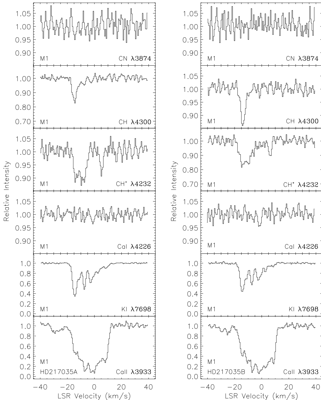
FIG. 14.—Interstellar CN, CH, CH + , Ca I, K I, and Ca II absorption profiles toward HD 217035A and HD 217035B (as for Fig. 1)
