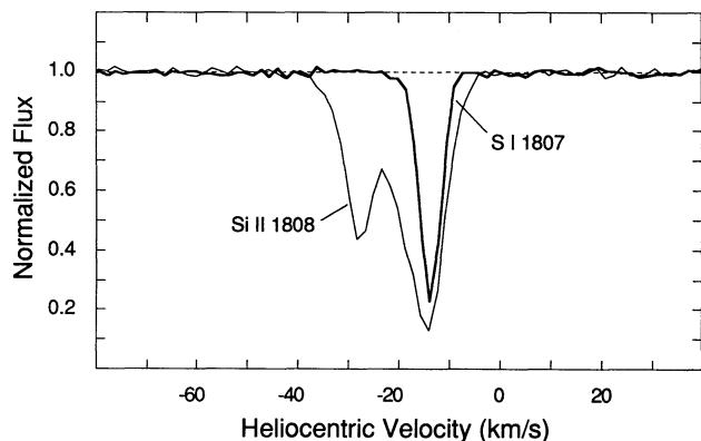
FIG. 1.—Echelle spectra for S I \lambda 1807 and Si II \lambda 1808. The strong S I line is only seen in the main component at -15 \text{ km s}^{-1} .
