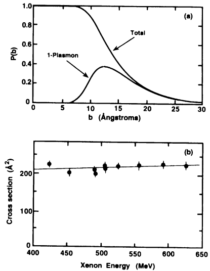
Fig. 4. (a) Calculated probabilities for the total interaction and for single-plasmon excitation as functions of the impact parameter, b , for 625 MeV ^{136}\text{Xe}^{35+} ions. (b) Calculated single-plasmon cross section (shown as a line) compared to the measured yields of C_{60}^+ from C_{60} bombarded by ^{136}\text{Xe}^{18+} ions in the energy range 420–625 MeV.
