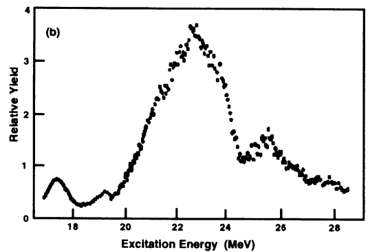
Fig. 3. Comparison of the giant dipole plasmon resonances observed in (a) the C_{60} molecule via photoionization with synchrotron radiation [9], and (b) the ^{12}\text{C} nucleus via the ^{11}\text{B}(p, \gamma)^{12}\text{C} reaction [11].
