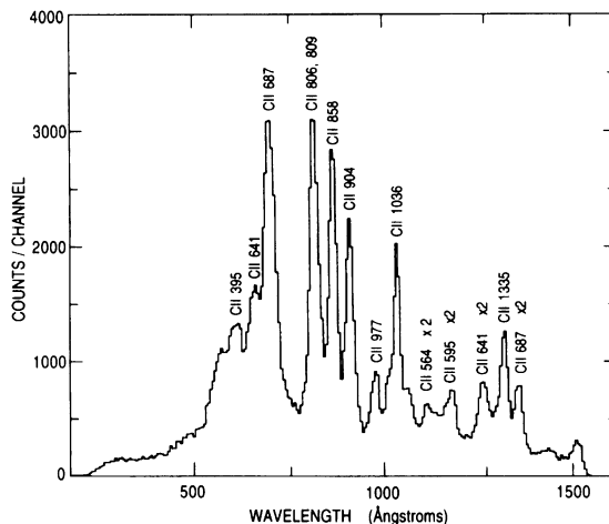
Fig. 6. VUV photon spectrum measured with a position-sensitive detector at the focal plane of a grating spectrometer located perpendicular to the incident beam direction. The xenon projectile energy was 625 MeV and the average charge state (after foil stripping just upstream of the C_{60} target) was 40+ . The peaks are labelled with identifications derived from the tabulations given in Ref. [17].
