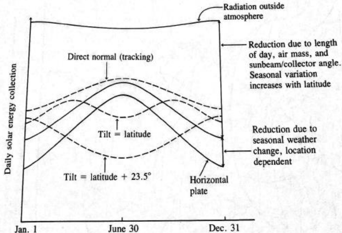
Figure 2.7 Qualitative plots of seasonal variations of daily solar energy collection for a location north of 23.5°N. "Tilt" (see Sec. 2.5) is the angle between the collector plate and the horizontal plane. The plate is tilted due south.
