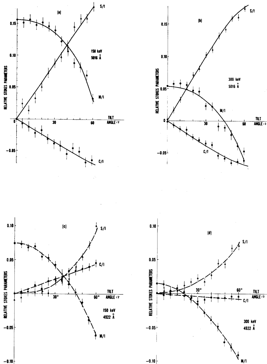
FIG. 1. Typical measurement of the dependence of the relative Stokes parameters upon foil tilt angle at selected energies. (a) 2s^1S-3p^1P (5016 Å) at 150 keV, (b) 2s^1S-3p^1P (5016 Å) at 300 keV, (c) 2p^1P-4d^1D (4922 Å) at 150 keV, (d) 2p^1P-4d^1D (4922 Å) at 300 keV. \bullet M/I , \blacksquare C/I , \blacktriangle S/I . Solid curve: fit to model of Band (Ref. 8); dashed curve: polynomial fit.
