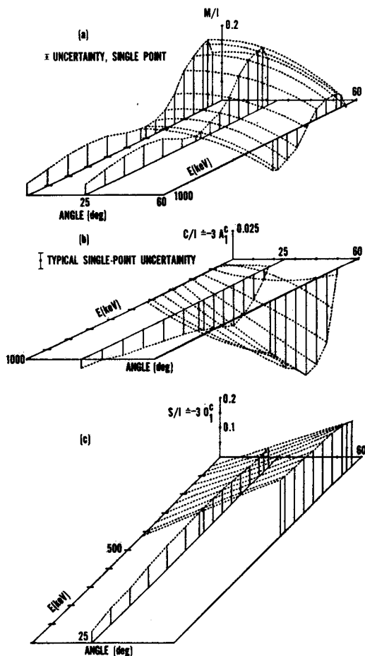
FIG. 2. Relative Stokes parameters for the transition 2s^1S-3p^1P at 5016 \text{ \AA} as a function of energy and angle. (a) M/I , (b) C/I \approx -3 A_1^c , (c) S/I \approx -3 O_1^c .
