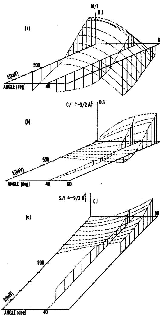
FIG. 3. Relative Stokes parameters for the transition 2p^1P-4d^1D at 4922 \text{ \AA} as a function of energy and angle. (a) M/I , (b) C/I \approx -\frac{3}{2} A_1^c , (c) S/I \approx -\frac{9}{2} O_1^c .
