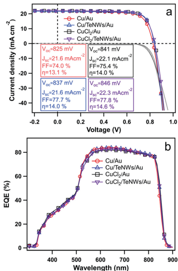
Fig. 5 (a) J - V characteristics and (b) external quantum efficiency (EQE) of CdTe solar cells with Cu/Au, Cu/TeNWs/Au, \text{CuCl}_2/\text{Au} and \text{CuCl}_2/\text{TeNWs/Au} back contacts respectively. The solid and dotted lines in Fig. 5(a) represent J - V curves under illumination and dark conditions respectively.
