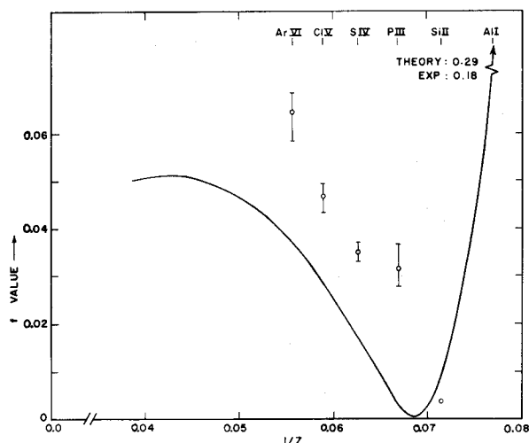
FIG. 2. Isoelectronic sequence for the Si II 3s^2 3p^2 P-3s 3p^2 D (see text concerning the ambiguity of this notation) transition. Experimental data sources are: Al I, Ref. 19; Si II, this work; P III, Ref. 20; Si IV, Ref. 21; Cl V, Ref. 22; and Ar VI, Ref. 23. The theoretical source is Ref. 18. An extensive set of figures of this type are given in Ref. 13.
