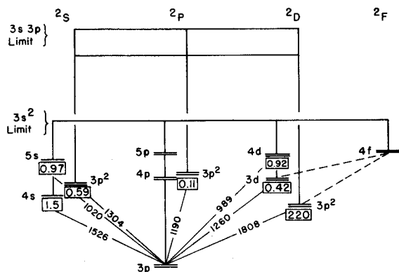
FIG. 1. Energy-level diagram for the low-lying levels of SiII. Levels are labeled by their dominant ls configuration and by our measured mean lives (boxed) in nsec, and resonance transition wavelengths are given in Å.
