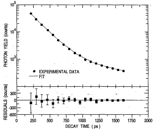
FIG. 3. Intensity decay data for the M1 peak. Upper curve is experimental data for one of three runs. The dotted line is a fit to a single exponential plus a power-law background. Lower curve is the residuals from the fit.
