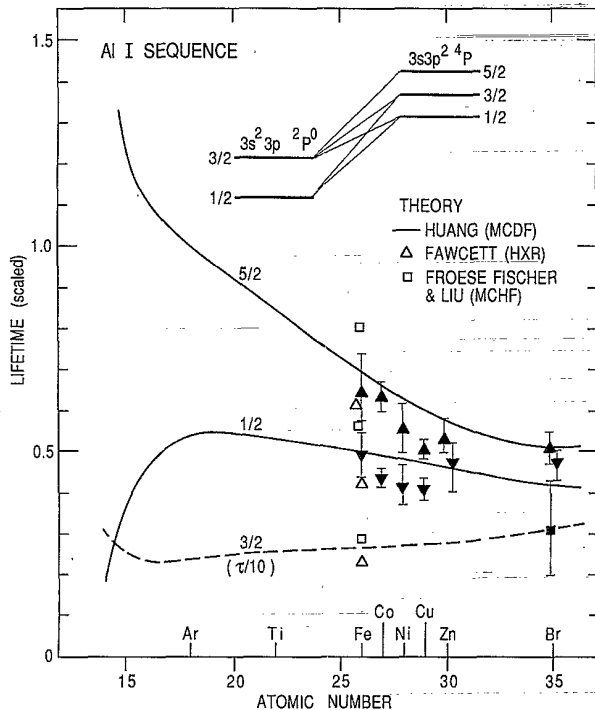
FIG. 4. Al I sequence: Scaled lifetime \tau of the 4P_j levels as a function of atomic number, Z . Theoretical values are taken from Refs. [40,41]. The vertical line displays the quantity [\tau(Z-10)^6 \text{ s}^{-1}] . The experimental data for the Br ion are from this work. Very recent work on \text{Si}^+ has been done by Calamai et al. [43] using an ion trap; these authors also discuss calculations done for very-low-charge-state ions.
