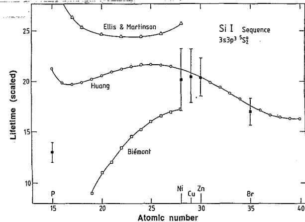
FIG. 5. Si I sequence: Lifetime [scaled as \tau(Z-10)^7 \text{ s}^{-1} ] of the 3s3p^3 \ ^5S_2 level. The only calculation for \text{Br}^{21+} is by Huang [37]. For references to calculations and experimental data at lower Z see Refs. [2] and Refs. [44–46] (calculations for P , S , and V ). The result for P^+ is from Calamai, Han, and Parkinson [42], who used an ion trap. All other experimental data are from beam-foil measurements.
