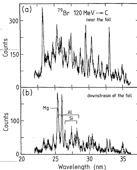
FIG. 2. Sample spectrum. (a) Sum of the spectra recorded near the foil, (b) sum of the spectra recorded away from the foil. The latter enhances the lines associated with decays of long-lived levels.
