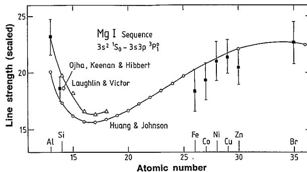
FIG. 3. Mg I sequence: Scaled line strength S as a function of nuclear charge (or atomic number). The quantity (S/10^{-6}\zeta^2) is displayed, where \zeta is the ionic core charge. The multiconfiguration relativistic random-phase approximation (MCRPRA) calculation extending to the Br ion is by Huang and Johnson [34], the low- Z theory by Laughlin and Victor [35] is based on a model-potential calculation. For discussions of theory and the result of a configuration-interaction calculation for Z = 14 see also Refs. [38,39].
