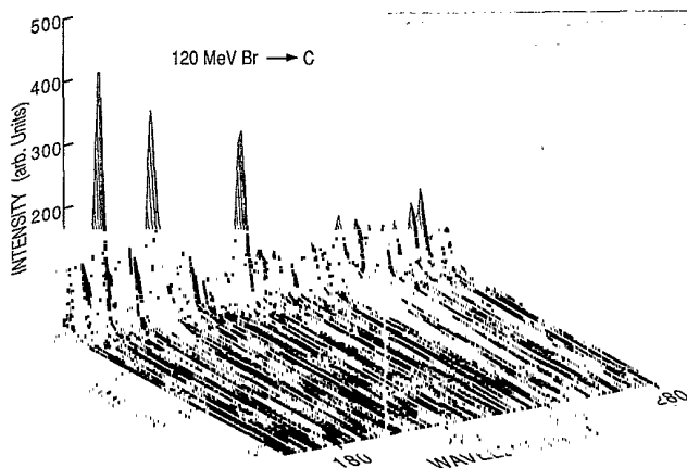
FIG. 1. Three-dimensional plot of spectra of bromine ions recorded at various foil positions. The presence of the decays of many short-lived levels in the spectra recorded close to the foil is evident; at longer times after excitation the few remaining lines are from the decays of long-lived intercombination transitions.
