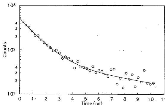
FIG. 3. Intensity decay for the 843.11-Å line in Hg III, 5d^{10}1S_0-5d^96p^3P_1 . The solid line denotes the two-exponential fit.
