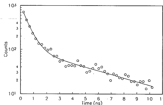
FIG. 2. Intensity decay for the 790.17-Å line in Hg III, 5d^{10}1S_0 - 5d^96p^1P_1 . The solid line denotes the two-exponential fit.
