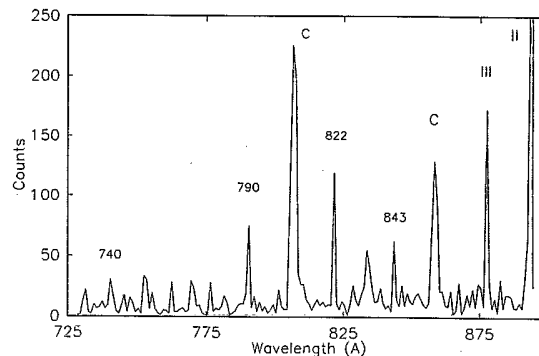
FIG. 1. Survey spectrum of Hg in the region 725–900 Å. The Hg III lines for which decay times were measured are indicated by wavelength. For a more detailed discussion of the spectrum, see text.
