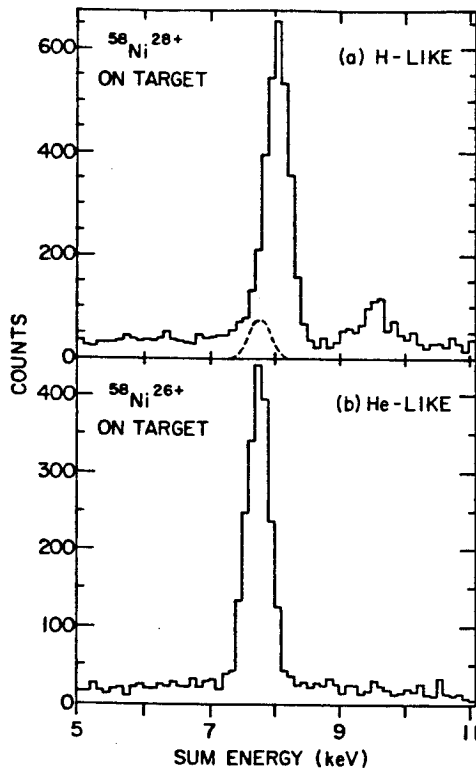
FIG. 2. Sum-energy spectra for true coincidences between one of the collimated Si(Li) detectors and the large solid-angle Si(Li) detector at the closest foil-detector distance. (a) Data taken with fully stripped \text{Ni}^{28+} incident on the target at 664 MeV. The peak near 8.0 keV is predominantly from two-photon sum coincidences from decay of the hydrogenlike 2^2S_{1/2} state. The dashed curve shows the contribution from heliumlike two-photon decays. The peak near 9.5 keV is due to true coincidences from n=3 \rightarrow n=2 \rightarrow n=1 cascades. (b) Data taken with heliumlike \text{Ni}^{26+} incident on the target at 664 MeV. The peak near 7.7 keV is predominantly from the two-photon decay of the heliumlike 2^1S_0 state of \text{Ni}^{26+} .
