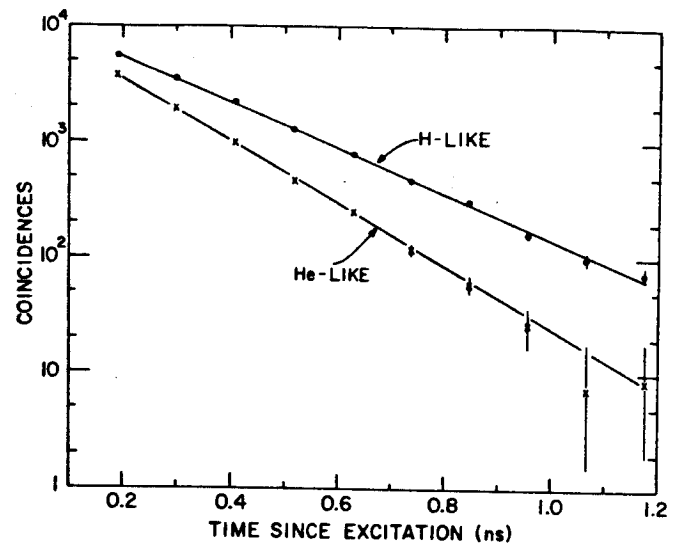
FIG. 3. Decay curves for two of the four lifetime measurements. These measurements were made with a ^{58}\text{Ni} beam of 664 MeV incident on a 12\text{-}\mu\text{g}/\text{cm}^2 foil in the target chamber. The data in the upper curve (solid dots) correspond to decays of the hydrogenlike 2^2S_{1/2} level in \text{Ni}^{27+} and were obtained with a fully stripped \text{Ni}^{28+} beam incident on the target. The data in the lower curve (crosses) correspond to decays of the heliumlike 2^1S_0 level in \text{Ni}^{26+} and were obtained with a \text{Ni}^{26+} beam incident on the target. The solid lines are two-component fits to the data (see text).
