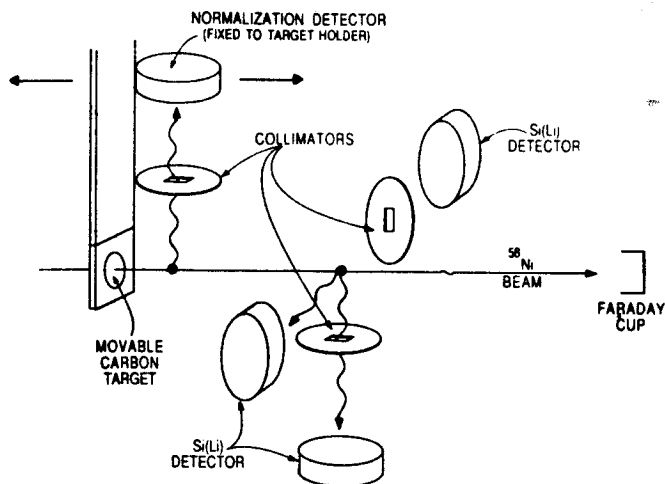
FIG. 1. Schematic diagram of the apparatus. The foil target is moved relative to three fixed Si(Li) detectors. Two of these detectors are collimated so that the detected photons are localized to a 5-mm region along the beam. A fourth lower-resolution x-ray detector, which moves with the target, is used for normalization.
