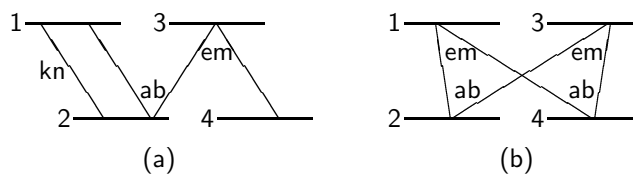
Figure 17.1. Illustration of methods for the determination of ratios of oscillator strengths.
